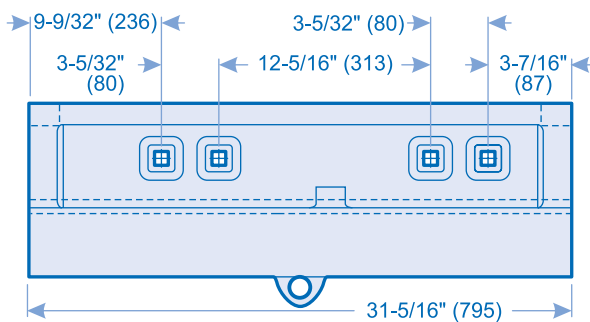
421-815-1211RCNR RH Center Edge (Shown - LH Opposite, 1 Ea. Req'd.) Weight - 111.0 lbs (50.4 kg.)
