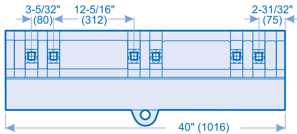
421-815-1211CNR (Center Edge, 1 Req'd.) Weight - 144.5 lbs (65.6 kg.)
