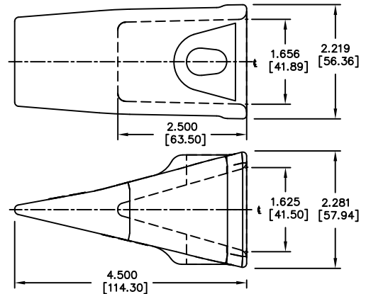
D7107319 1.9 lbs. (0.86 kgs.) (bolt & nut available soon)
