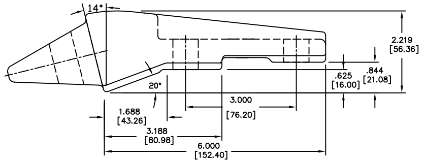
D6737324 5.2 lbs. (2.36 kgs.)
