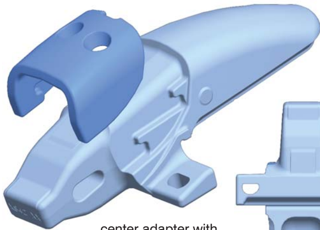
center adapter with replaceable wear cap
